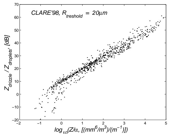
Fig. 3. The dependence of the drizzle to droplets reflectivities ratio versus the ratio of radar reflectivity to optical extinction Z/\alpha for CLARE'98 data.
