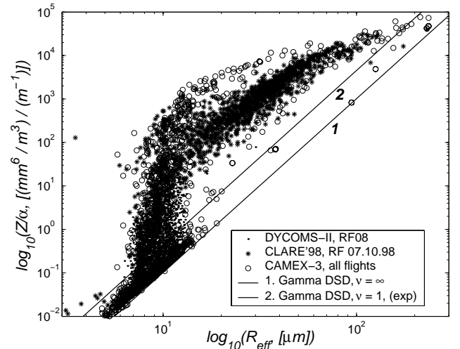
Fig. 5. The Radar to Lidar Ratio versus the Effective Radius for the CLARE'98, DYCOMS-II, and CAMEX - 3 campaigns data
