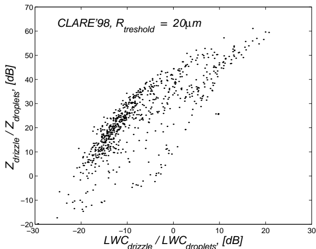
Fig. 1. The dependence between the ratio of drizzle to droplets reflectivities versus the ratio of drizzle to droplets LWCs for CLARE'98 campaign data.
