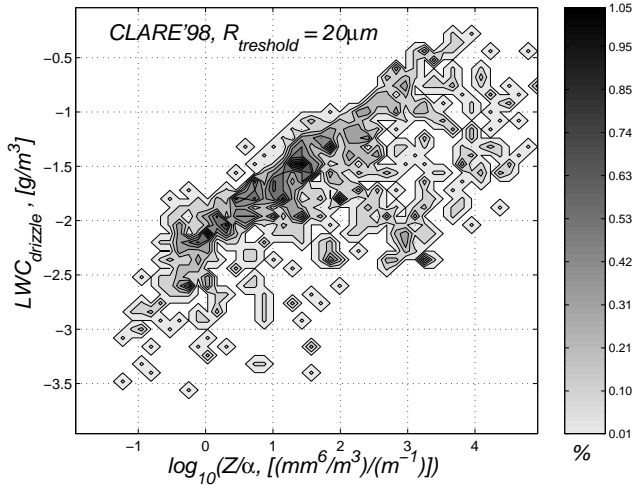
Fig. 4. The dependence of the LWC in drizzle fraction versus the Z/\alpha ratio for CLARE'98 data.
