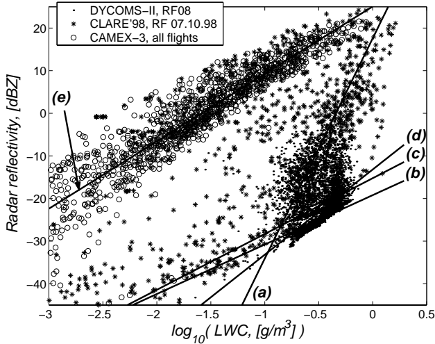
Fig. 6. The relation between Liquid Water Content and Radar Reflectivity for different field campaigns. Lines represent the different linear fittings of this relation.
