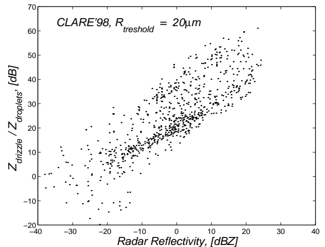
Fig. 2. The dependence of the ratio of drizzle to droplets reflectivities versus total radar reflectivity for CLARE'98 campaign data.
